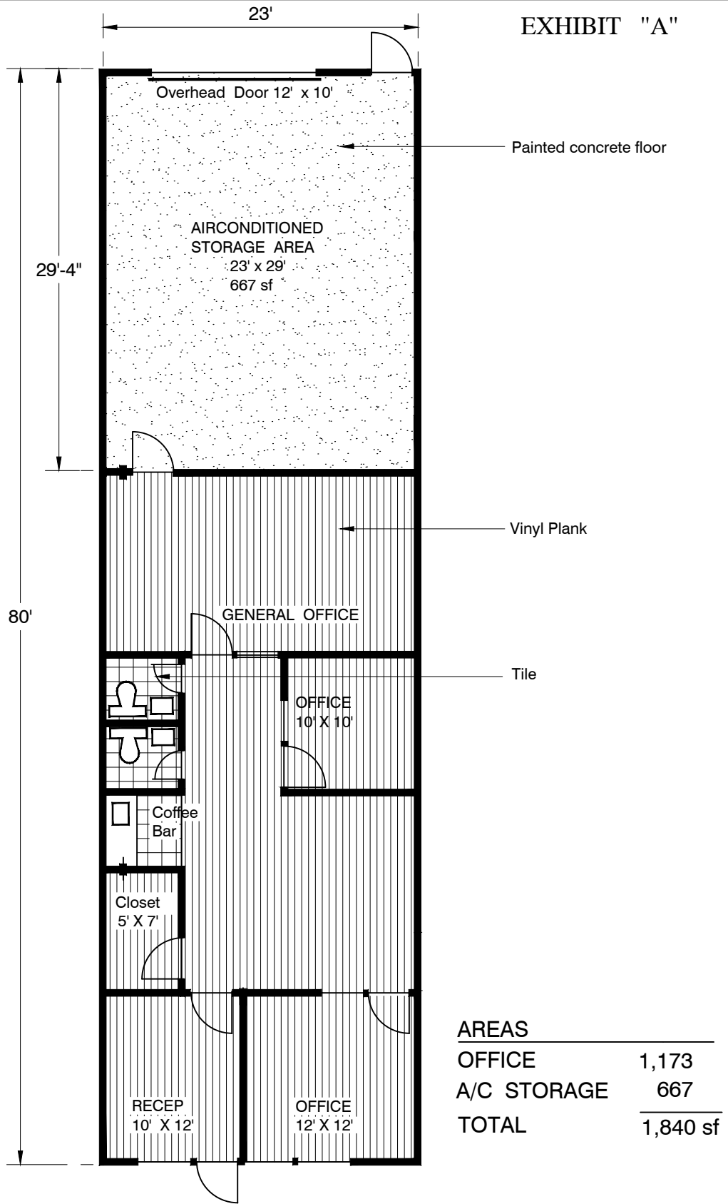
FLOOR PLAN of 1774 W SAM HOUSTON PARKWAY N
